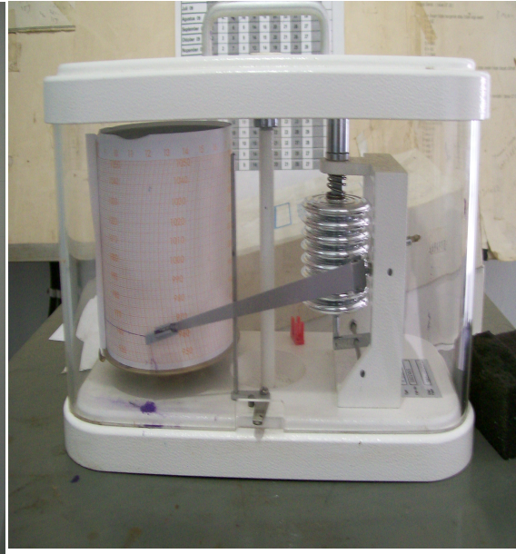
Gambar Barograph
